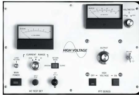
PFT-503CM Control Layout
